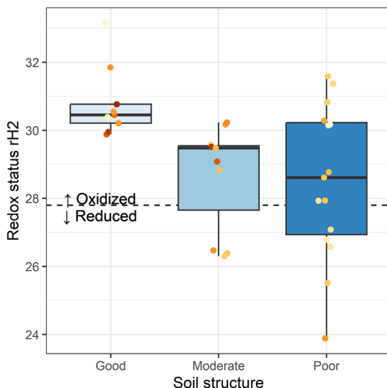
Fig. 4 The redox status (rH2) of soils with a good structure (VESS 1–2.75) was more oxidized than soils with a poor structure (VESS 3.25–5). The colors on the points describe the soil OM concentration (Fig. 1 legend)
