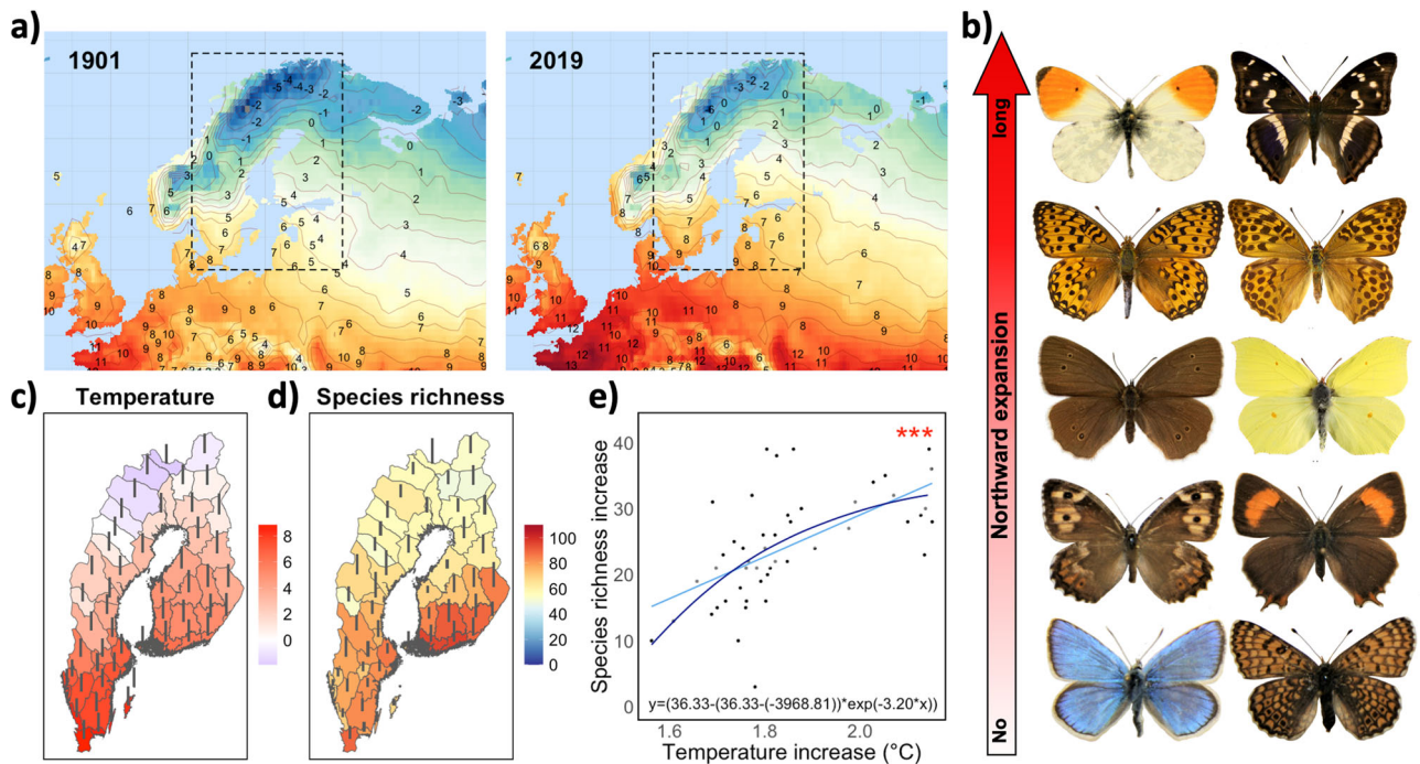
Fig. 1 Changes in species richness and temperature from 1901 to 2019 in the study area and examples of butterfly study species. The two top left panels (a) show mean annual temperatures in (parts of) Europe in 1901 and in 2019. The right panel (b) shows examples of study species sorted from bottom to top according to their northward range expansion (from no to long). Polyommatus dorylas , Melitaea cinxia , Hipparchia semele , Thecla betulae , Aphantopus hyperantus , Gonepteryx rhamni , Speyeria aglaja , Argynnis paphia , Anthocharis cardamines and Apatura iris (Photos by Vladimir Kononenko, reprinted with permission from copyright holder Leif Aarvik). The bottom panel, (c) shows current temperature (°C, indicated by colour) and temperature change (1901–2019) indicated by the length of the bar for each of the 51 provinces in Sweden and Finland, (d) shows current species richness (colour) and change (1901–2019) in species richness (length of the bar), and (e) shows the linear (light blue line) and asymptotic (dark blue line) increase in species richness with temperature increase from 1901 to 2019. Each dot represents one province ( n = 48 ).
