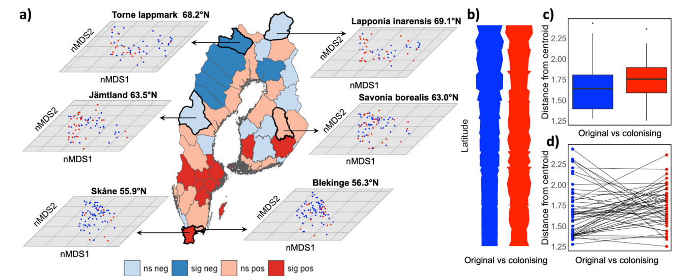
Fig. 5 Comparison of within-group variability of trait values between the original community and the colonising species. Within-group variability was estimated (using the PERMDISP implementation in the ‘vegan’ package in R) as the mean dispersion from the centroid based on data of the continuous numeric variables body size (wingspan), species mean temperature, species temperature range, and distribution range size. Left panel (a) shows the PERMDISP results from within-province comparisons. Colours in the map indicate whether trait variability was higher in original (blue) (northern) or colonising species (red) (south central), and shades indicate whether the pairwise test was significant (darker shade) or not (lighter shade). Colours in the nMDS plots for a subset of the provinces at three latitudes are blue: original species, red: colonising species. In (b) the blue and red vertical bars show the association of within-group trait variability with latitude (wider bars indicate higher trait variability) in the original community (blue) and in the group of newly established species (red). Scatterplots of these relationships are available in Figure S5. The upper right panel (c) shows the overall result from the paired comparisons of within-group trait variability (distance from centroid) between original and colonising species in each province. Boxes indicate interquartile range (IQR), vertical line denote median, upper and lower whisker third quartile +1.5 × IQR and 1st quartile −1.5 × IQR range, and dots represent outliers. The lower right panel (d) shows the heterogeneity of the outcomes of the province-based pairwise comparisons.
