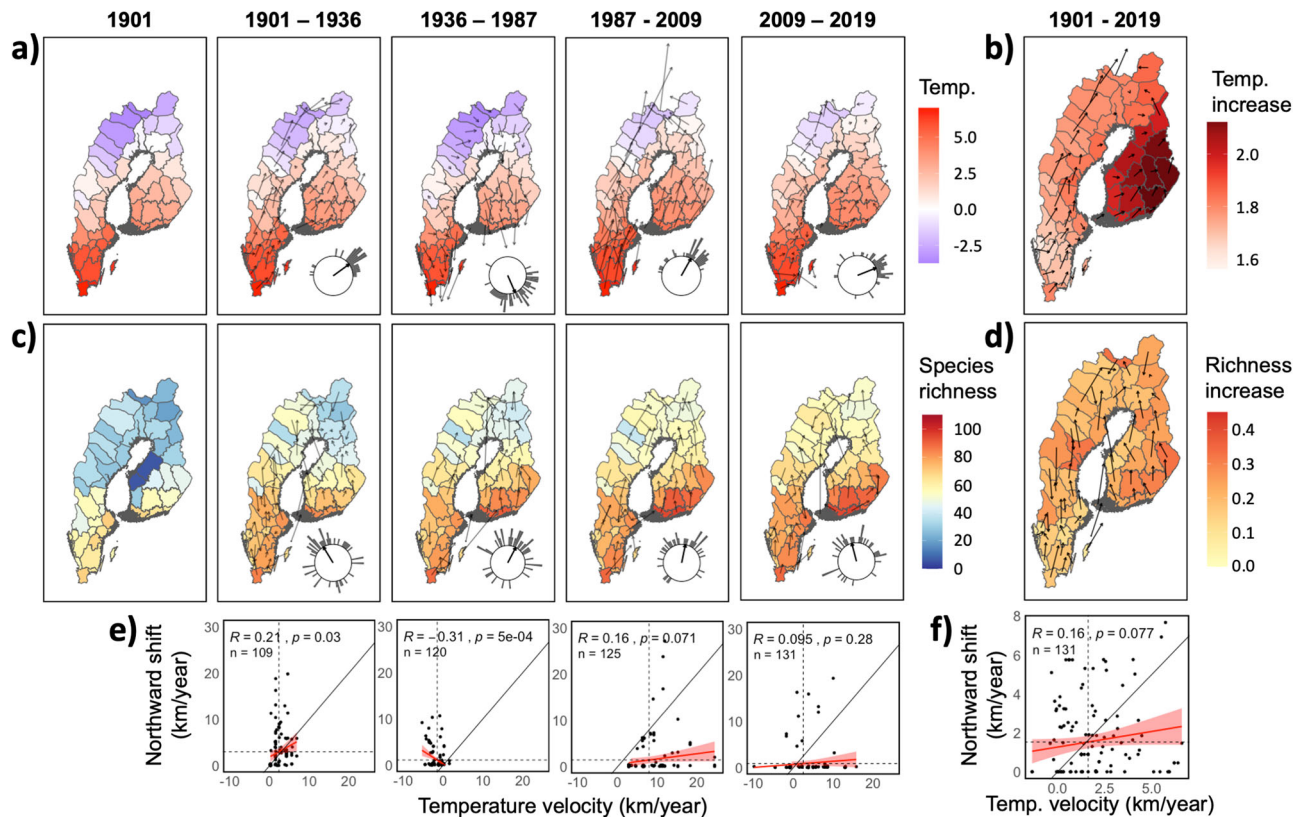
Fig. 2 Temperature, average temperature movements, species richness, average species movements, and associations between northward range shifts and northward temperature shifts in four periods during the past 120 years (from 1901 to 2019). Colour codes in the top maps indicate spatial variation in (a) temperature (°C) for each timepoint, and in (b) temperature increase (°C) over the entire study time range (1901–2019). Colour codes in the lower maps indicate spatial variation in (c) species richness for each timepoint and (d) species richness increase (species per year) over the entire study time range (1901–2019). Arrows in maps represent mean province based movement per period and over the entire study duration for mean annual temperature (a and b), and species richness (c and d). Circles in (a) indicate the distribution of mean direction of province-based temperature movements (bars, where 0° is north with rotation clockwise, and length of bar indicate the number of observations), and needles from centres indicate the average mean across provinces. Circles in (c) indicate the distribution of mean direction of province-based species movements (bars, where 0° is north with rotation clockwise, and length of bar indicate the number of observations), and needles from centres indicate the average mean across provinces. The bottom row shows associations between northward species range shifts (km/year) and northward temperature shifts (km/year) for (e) each period separately and (f) for the entire study duration. In (e) and (f), each species contributed one measure of northward range shift velocity per period (calculated as the northward distance (km) between the northernmost province of a species distribution from one time point to the next divided by the duration of the period (in years), for details see Methods), and the corresponding temperature shifts were extracted based on the starting coordinates (longitude and latitude) of each range shift (for details see Methods). n -values denote sample sizes, which increased for each period as new species were observed (colonised the study area). Diagonal lines indicate the isometric relationship expected if the rate of species northward range shifts coincide with the rate of temperature shifts. Red lines with shaded areas represent regression lines with 95% confidence intervals. Observations for species with zero northward range expansion have been jittered along the y-axis. R -values denote Pearson correlation coefficients.
