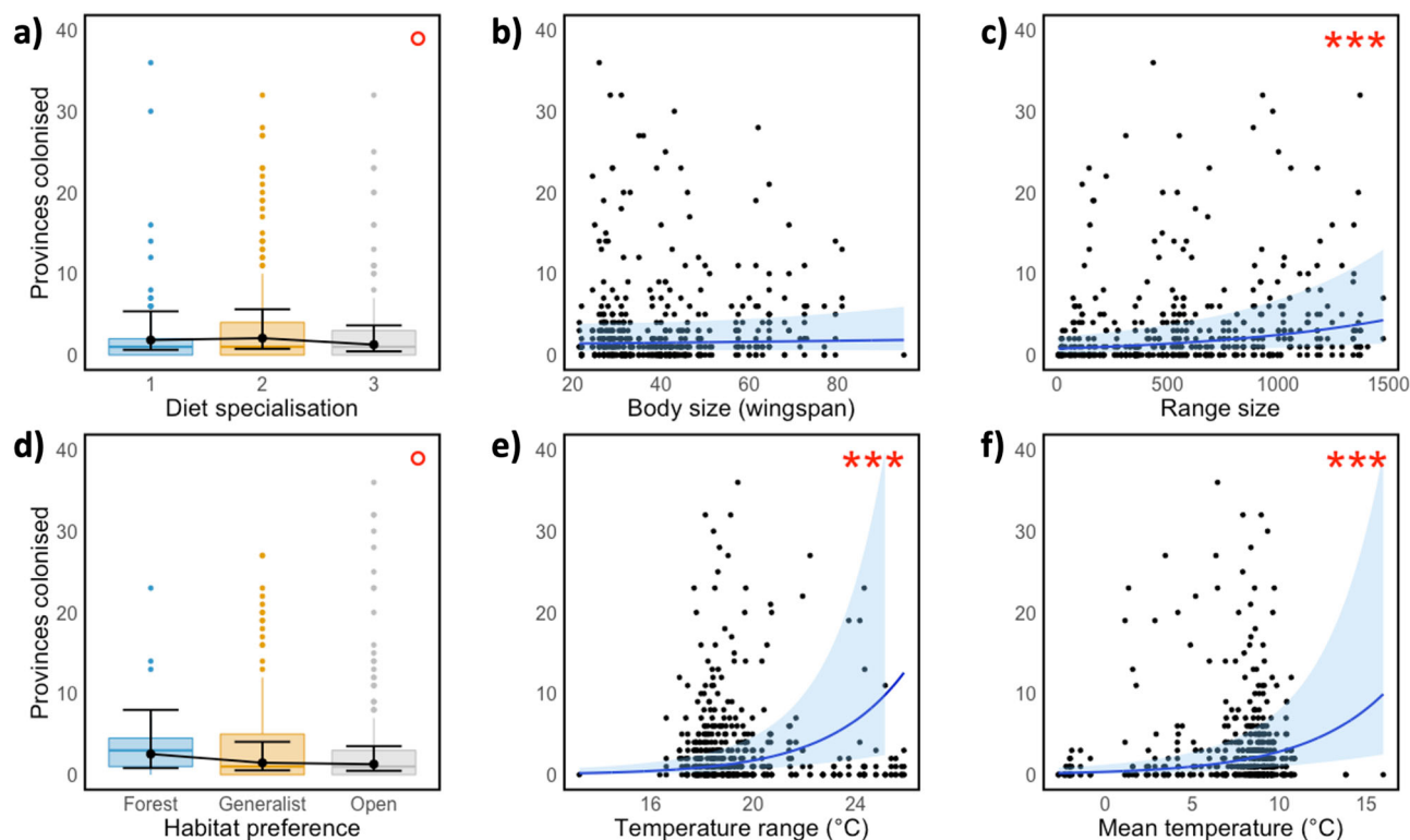
Fig. 4 Associations of establishment success of butterflies with species traits. Figures are based on the GLMM and raw data illustrating the number of new provinces the species colonised as a function of (a) diet specialisation (where 1 = monophagous, 2 = oligophagous, and 3 = polyphagous), (b) body size (wingspan), (c) total range size, (d) habitat preference, and thermal niche quantified as (e) mean species temperature index, and (f) range of the species temperature index. Each dot represents one species and one period. The coloured box plots (in a and d) are based on raw data and boxes indicate the first and third quartiles, horizontal lines indicate the median, vertical lines indicate 1.5 \times \text{IQR} , and coloured dots indicate outliers. Overlaid in black (a and d) are least-squares means with associated error bars from the GLMM reported in Table 1b. In panels b, c, e, and f, the black dots represent raw data (each dot representing one species and one time period), and the blue lines and shaded areas show the predicted mean lines with 95% CI obtained from the GLMM ( n = 467 ) reported in Table 1b. ^{\circ}0.05 < P < 0.1 , ***P < 0.001 , see Table 1b and Table S2 for details.
