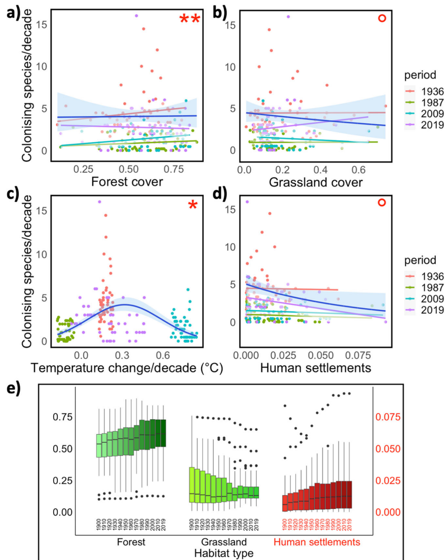
Fig. 3 Associations of variation in provincial colonisation rate of butterflies with land use and temperature change. Scatterplots show provincial colonisation rate (number of colonising species per decade) as a function of (a) forest cover, (b) grassland cover, (c) temperature change, and (d) human settlements. Each dot represents data for one province per period with different colours of the dots for each of the four time periods. Dark blue lines and blue shading illustrate the predicted mean lines with 95% CI obtained from the GLMM ( n = 201 ). The thin trend lines of different colours represent the associations based on linear regressions as estimated separately for each of the four time periods. Red asterisks indicate significant interactions with time period, ° 0.05 < P < 0.1 , * P < 0.05 , and ** P < 0.01 , see Table 1a and Table S1 for details. Bottom panel (e) shows how the proportion of each habitat type changed over time (one box every 10th year between 1900 and 2010, and one box for 2019). Each province contributes one value per time point. Boxes indicate interquartile range (IQR), vertical line denote median, upper, and lower whisker third quartile +1.5 \times \text{IQR} and 1st quartile -1.5 \times \text{IQR} range, and dots represent outliers. Note that the scale on the vertical axis is different for human settlements. Data for (e) were obtained from the HILDA GIS product 102-104 .
