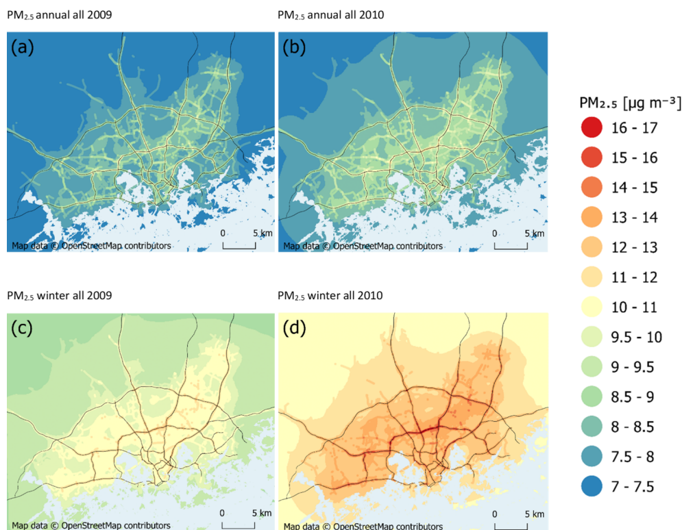
Figure 4. The predicted average concentrations of PM 2.5 ( \mu\text{g m}^{-3} ) in the Helsinki region, as annual averages in (a) 2009 and (b) 2010 and as winter averages in (c) 2009 and (d) 2010. The main street and road network are presented with the black lines, and the sea areas are in a light-blue colour. The physical scales of figures are indicated by the bars on the lower right-hand sides of each panel. © OpenStreetMap contributors 2019. Distributed under the Open Data Commons Open Database License (ODbL) v1.0.
