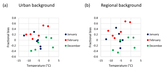
Figure C1. Fractional bias of the computations for the winter months as a function of the ambient temperature for the (a) urban- and (b) regional-background stations. A positive bias corresponds to a model over-prediction. The data include all the years targeted in this study.
