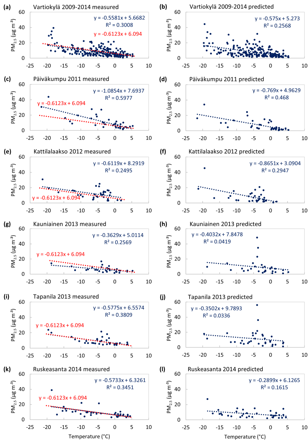
Figure 3. Daily average measured (left-hand side panels) and predicted (right-hand side panels) concentrations as a function of the ambient temperature. The data have only been presented for the cases in which the contribution attributed to RWC was above the average value at the residential stations. The linear trends of data in each figure have been presented by the blue lines. The overall average trend of observed concentrations on temperature for all years and stations is presented by the red lines; this trend is therefore the same for all the panels on the left-hand side.
