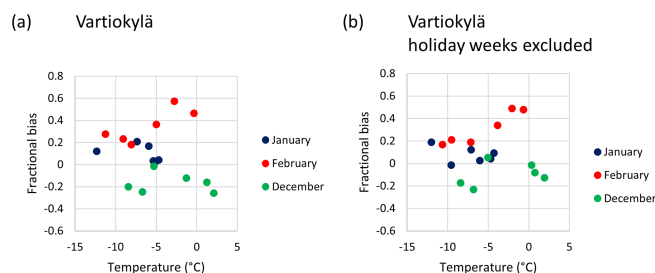
Figure C2. Fractional bias of the computations for the winter months as a function of the ambient temperature for the permanent residential station of Vartiokylä. Panel (a) presents all the considered data, and panel (b) presents all the data except for that during the holiday weeks in winter. A positive bias corresponds to a model over-prediction. The data include all the years targeted in this study.
