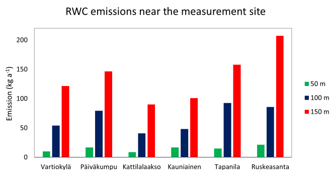
Figure B1. The modelled total amounts of emissions originating from RWC near the residential measurement sites. The legend indicates different radial distances from the measurement site.
