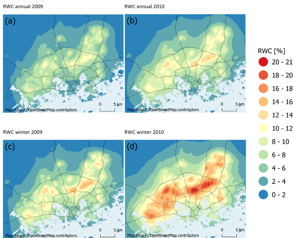
Figure 5. Contribution of residential wood combustion to the concentrations of PM 2.5 (a, b) annually and (c, d) in winter in 2009 and 2010 (%). © OpenStreetMap contributors 2019. Distributed under the Open Data Commons Open Database License (ODbL) v1.0.
