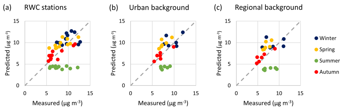
Figure 2. Predicted and measured concentrations ( \mu\text{g m}^{-3} ) during the seasons of the year for three categories of stations, i.e. residential and urban and regional background, during 2009–2014.
