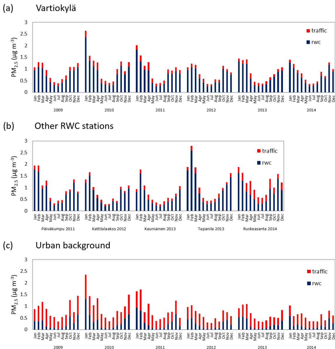
Figure 6. Predicted monthly average concentrations originating from urban sources, attributed to urban vehicular traffic and residential wood combustion. The regional background has been excluded.
