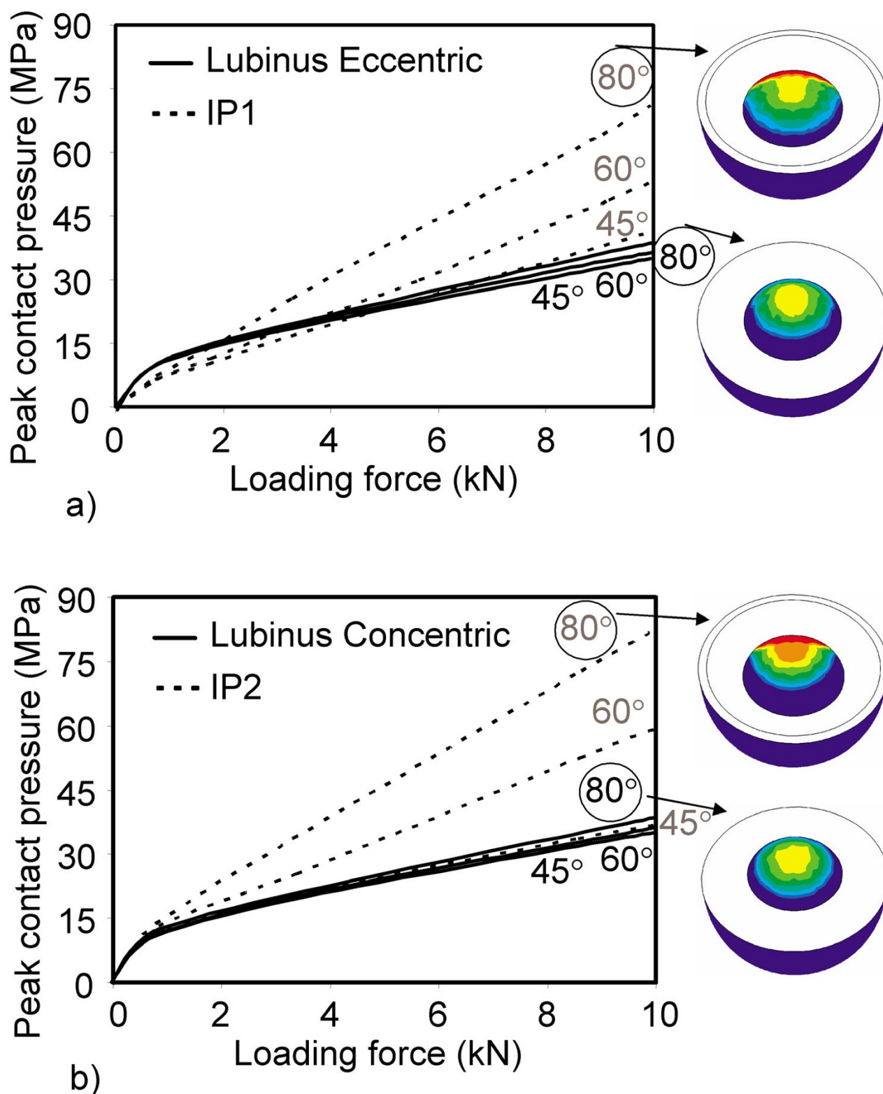
Figure 5 Peak contact pressure at the cup-head interface as a function of loading force and abduction angle. a) Lubinus eccentric and IP1, b) Lubinus concentric and IP2.
