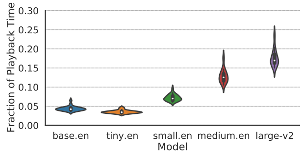
Figure 4: Relative transcription time. If the playback time is 50 s and it takes 10 s to generate the transcript then the fraction of playback time is 10/50 = 0.2, i.e., generating a transcript required 20% of the playback time. (Range = min, max)
