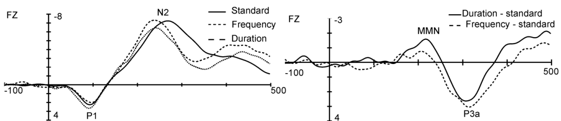
Figure 5. Grand average waveforms of the ERP responses elicited by the standard tone and deviant tones (left), and deviant-minus-standard subtraction waveforms for the duration and frequency deviant tones (right)
