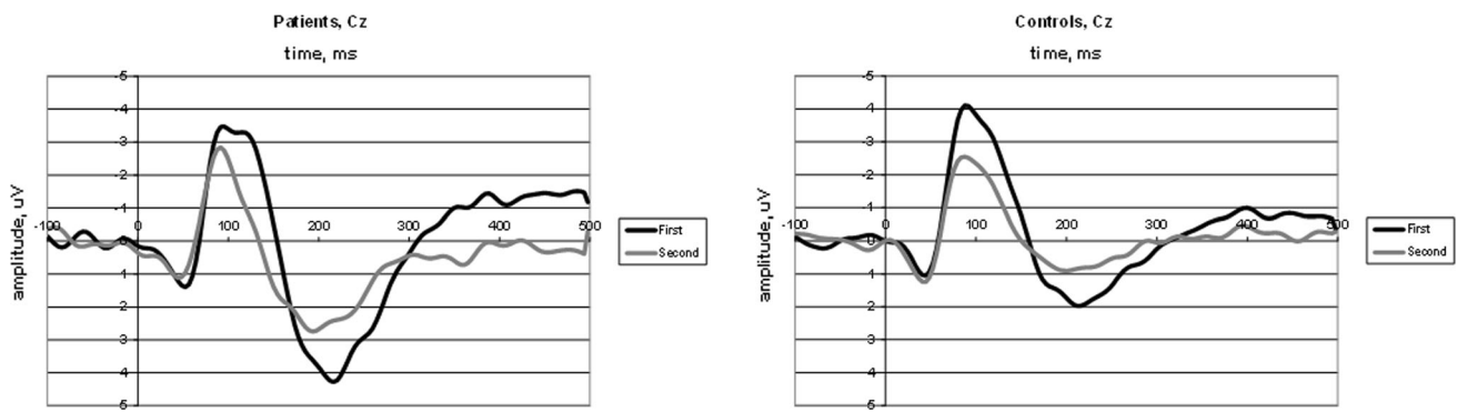
Fig. 1 Auditory event-related potentials in response to the first ( black ) and second ( gray ) tone of a pair of tones (ISI 0.5s) measured at the central (Cz) electrode location
