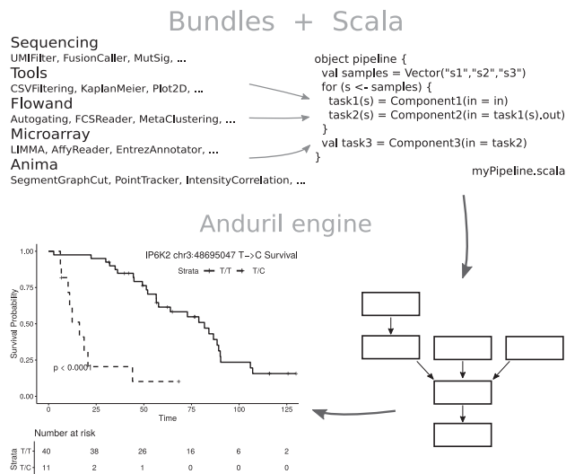
Fig. 1. Anduril 2 overview. Many common pre-processing and downstream analysis steps have been encapsulated in components coded in a variety of supported languages (R, Matlab, Python, Java). Components are organized in bundles dedicated to specific datasets (anima—image processing, flowand—flow cytometry, sequencing—omics data, tools—general, microarray) and are combined into pipelines in a Scala program run by the Anduril engine. Anduril constructs a graph and handles execution of the pipeline tasks in parallel while keeping track of the changes and status (pass/fail) of different steps to ensure reentrancy. The Kaplan-Meier curve shown here is a direct output of the case study and shows the survival difference in the TCGA ovarian patients with a T/C genotype in IP6K2 gene (chr3: 48695047, P -value 0.0001)
