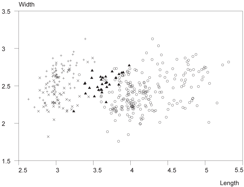
Fig. 2. Spore measurements ( \mu\text{m} ) comparing Trechispora elongata ( \circ ) with T. caucasica ( \blacktriangle ), T. farinacea (+) and T. stevensonii ( \times ). Each symbol represents a single spore. The points have been jittered, i.e. moved randomly within 0.05 \mu\text{m} around the original value along both axes.
