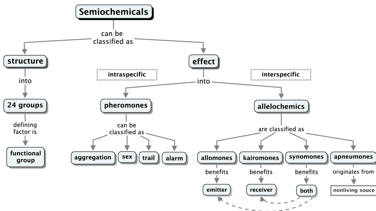
Figure 1. The classification of semiochemicals.
