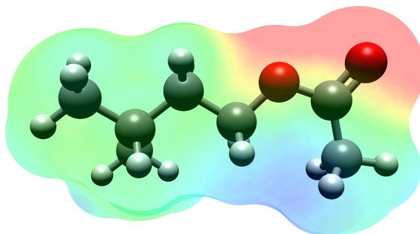
Figure 2. Molecular model of isopentyl acetate
