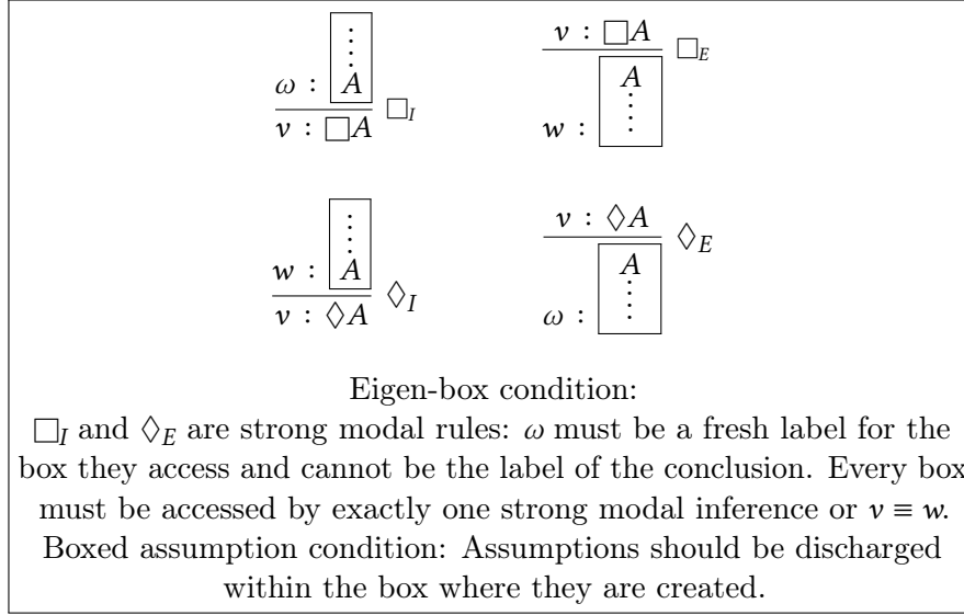
Figure 3: Modal rules
