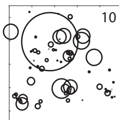
TA = x2, NP, PC = original, PD = originalx2, MA = x2
