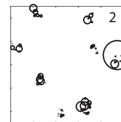
TA, NP, PD, MA = original, PC = clust8
