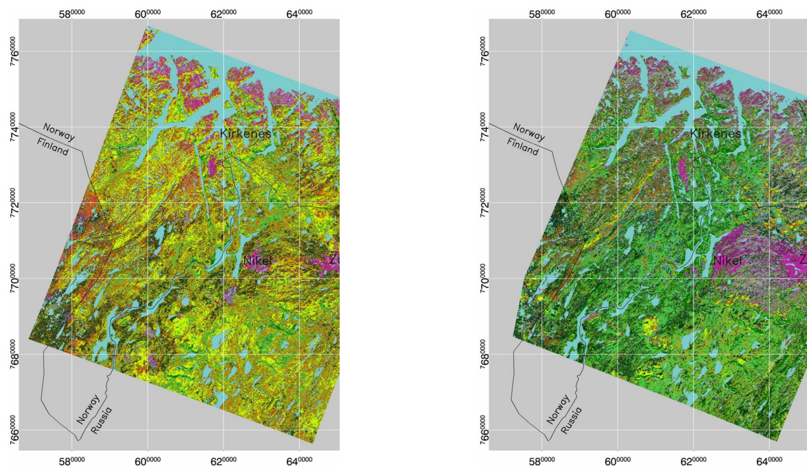
Figure 4.22 Land cover maps based on Landsat imagery of the study area. Damaged areas are shown in red to violet colour, and lichen-dominated forests and alpine heaths are yellow to green. The map shows the situations in 1973 and in 1999.
