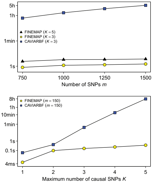
Fig. 3. Processing time of one locus with FINEMAP and CAVIARBF on \log_{10} scale. Top panel: Scenario A with increasing number of SNPs allowing K = 3 or K = 5 causal SNPs. Bottom panel: Scenario B with 150 SNPs considering causal configurations with different maximum numbers of SNPs. All processing times are averaged over 500 datasets using one core of a Intel Haswell E5-2690v3 processor running at 2.6 GHz
