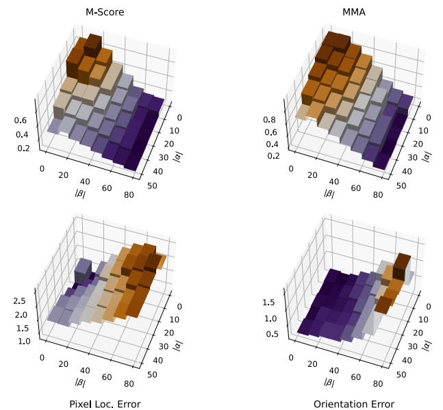
FIGURE 8. Synthetic data: LAFE median performance versus changes in lighting in degrees. See text for details.
