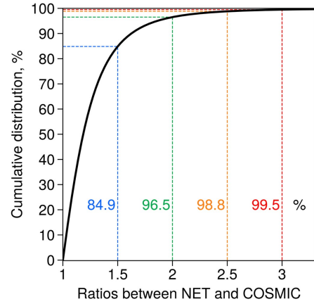
b Ratios between NET predictions and COSMIC data
