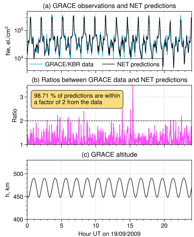
Figure 3. (a) In-situ GRACE observations and NET predictions on 19 September 2009 (note that this day was not used for model training and belongs to the test interval), (b) Ratios between the model predictions and the data, (c) GRACE altitude.
