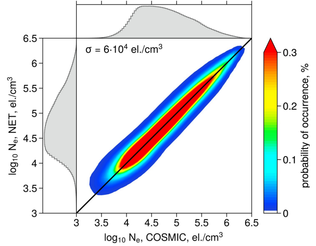
b Ratios between NET predictions and COSMIC data
