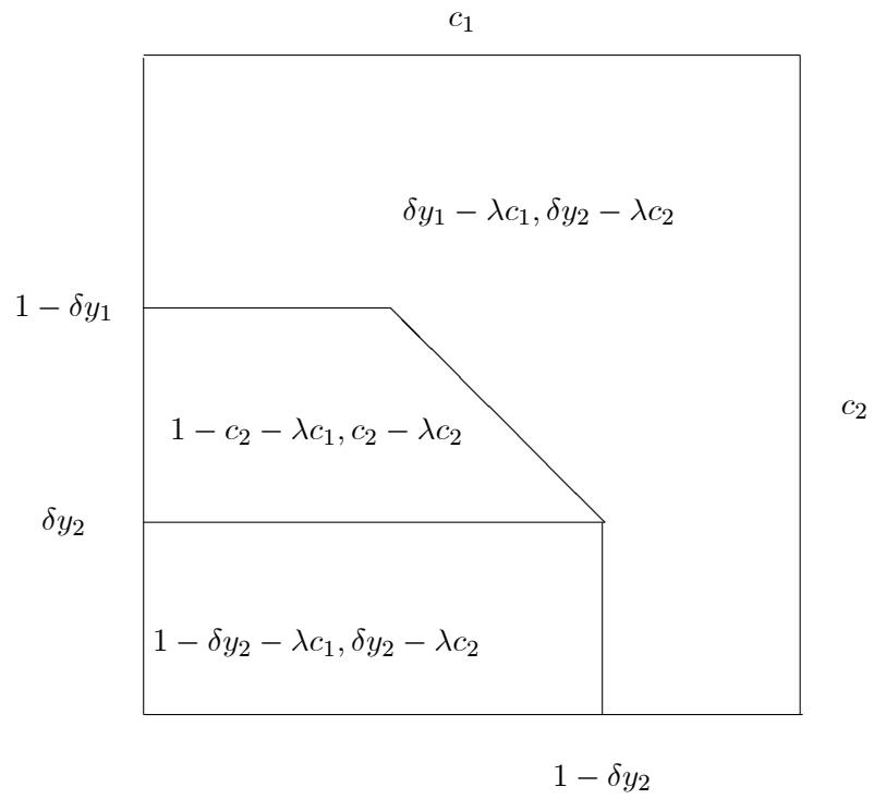
Figure 1: The case of one round: Subgame perfect equilibrium utilities after every pair (c_1, c_2)
