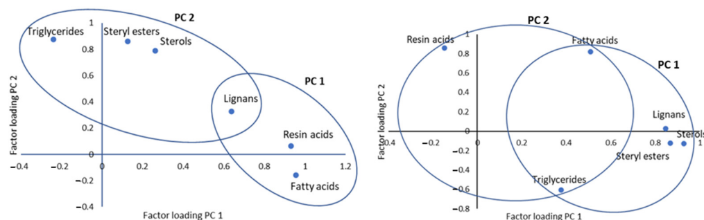
Figure 5. Factor loadings of compounds of Scots pine stem wood from final-felling and thinning trees ( left ) and all biomass components ( right ) generated by principal component analysis. Compounds belonging to PC 1 and 2 are marked by circles.
