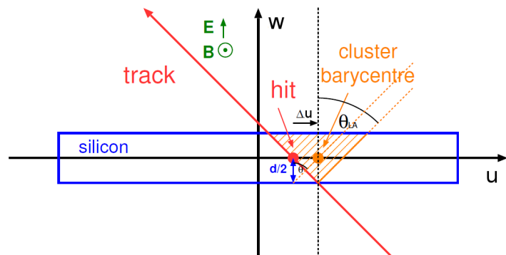
Figure 7. Illustration of the Lorentz angle. Due to the magnetic field, charge carriers in the silicon drift to the direction indicated by orange lines, with an angle with the electric field lines called the Lorentz angle. As a result, the cluster barycentre is reconstructed in a biased position, unless the Lorentz effect is properly accounted for.
