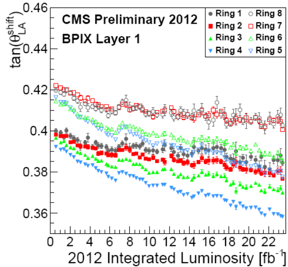
Figure 9. Evolution of the Lorentz angle in 2012 for 8 rings of layer 1 of the pixel barrel.
