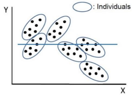
Figure 4. The hypothetical scatter plot for the relation between X and Y in a model with random slopes . Dots present data points and individuals are circled. If the individual differences in within-person relations are not addressed, the positive and negative effects may cancel each other out and produce a non-significant overall effect on the between-person level (the blue line).
