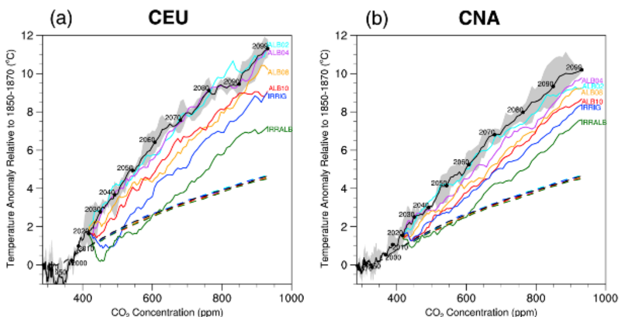
Figure 3.22: Regional temperature scaling with carbon dioxide (CO 2 ) concentration (ppm) over 1850 to 2099 for two different regions as defined in the Special Report on Managing the Risks of Extreme Events and Disasters to Advance Climate Change Adaptation (SREX): Central Europe (CEU) (a) and Central North America (CNA) (b). Solid lines correspond to the regional average annual maximum daytime temperature (TX x ) anomaly and dashed lines correspond to the global mean temperature anomaly, where all temperature anomalies are relative to 1850–1870 and units are degrees Celsius. The black line in all panels denotes the 3-member control ensemble mean with the grey shaded regions corresponding to the ensemble range. The colored lines correspond to the 3-member ensemble means of the experiments corresponding to albedo
