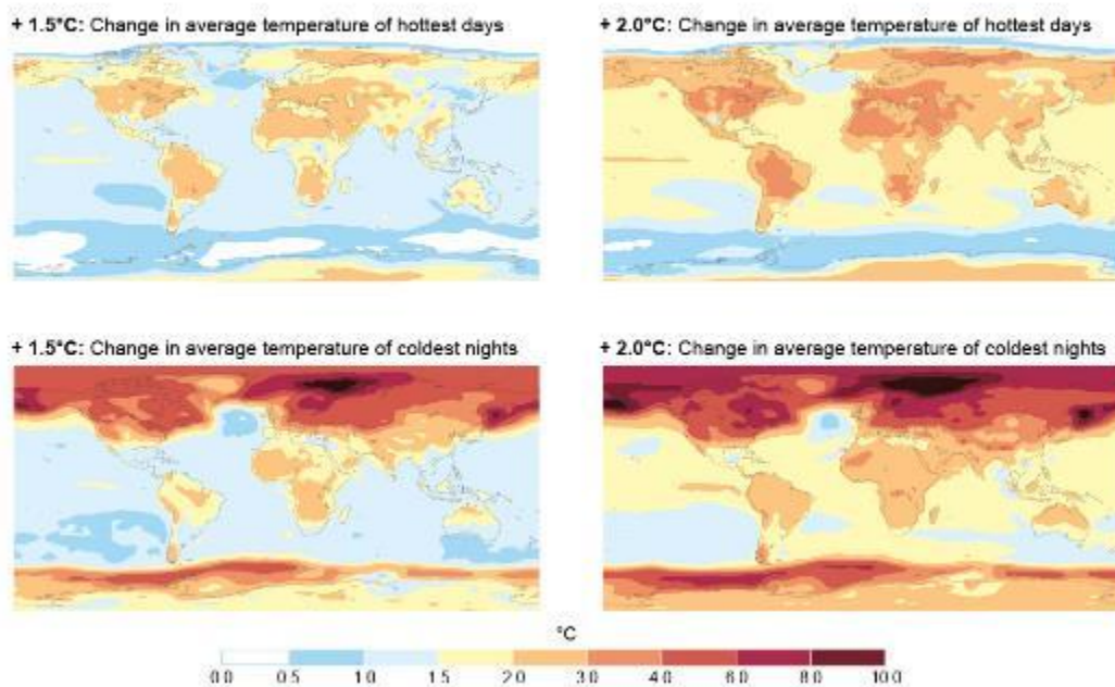
FAQ 3.1, Figure 1: Temperature change is not uniform across the globe. Projected change in average temperature of the annual hottest day (top) and the annual coldest night (bottom) with 1.5°C global warming (left) and 2°C global warming (right) compared to pre-industrial levels.
