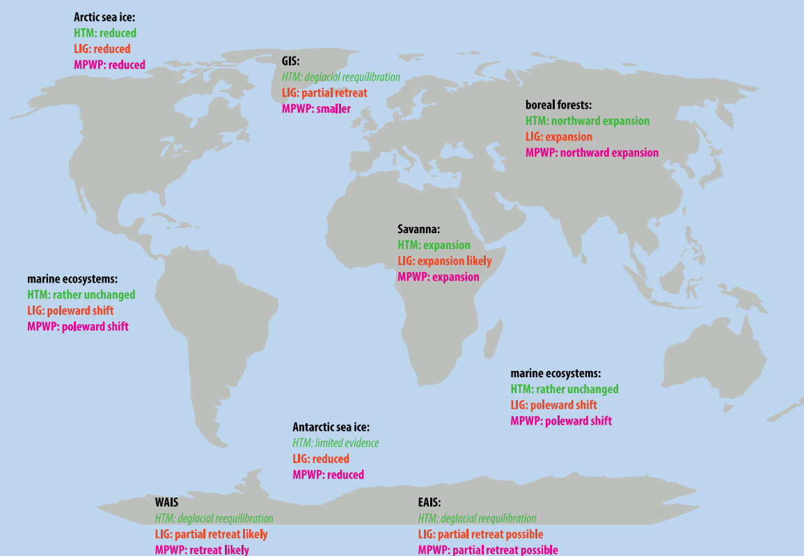
Box 3.3, Figure 1: Impacts and responses of components of the Earth System. Summary of typical changes found for
