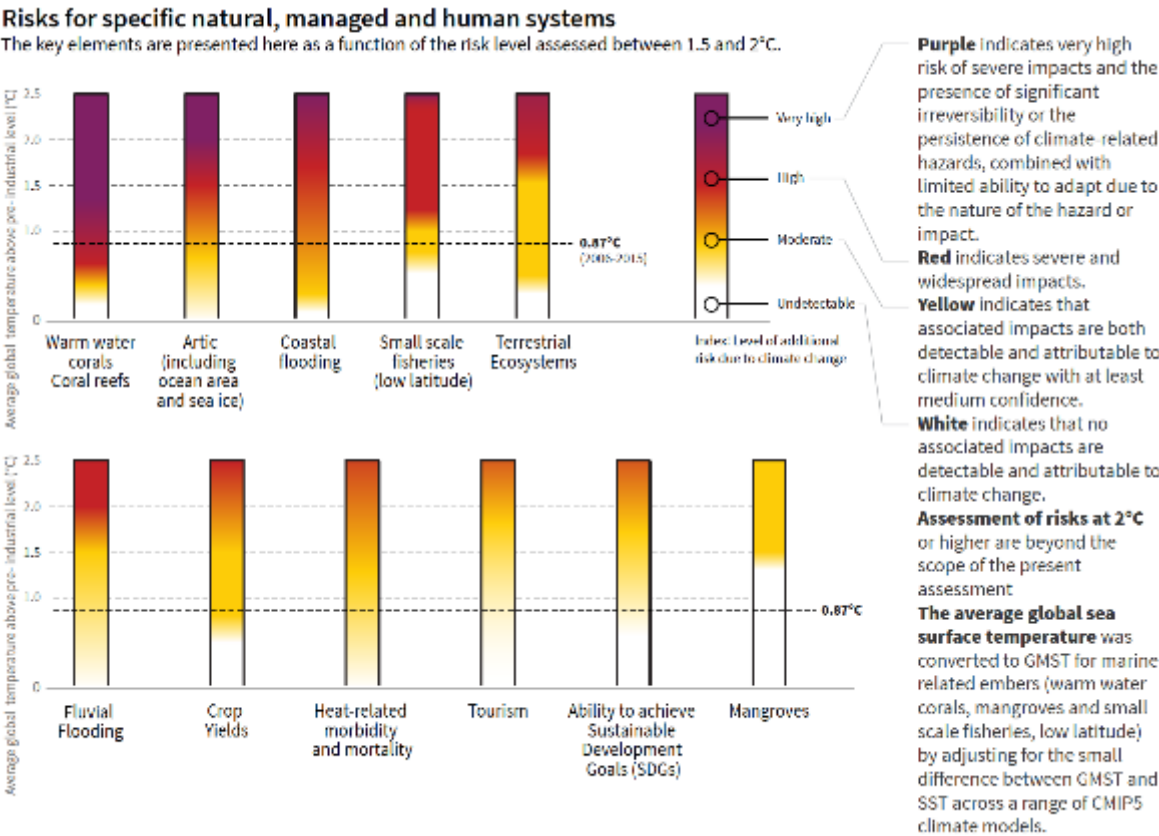
Figure 3.20: The dependence of risk associated with selected elements of human and natural systems on the level of climate change, adapted from Figure 3.18 and from AR5 WGII Chapter 19, and highlighting the nature of this dependence between 0 and 2°C warming above pre-industrial levels. The color scheme indicates the additional risks due to climate change. The shading of each ember provides a qualitative indication of the increase in risk with temperature for each individual ‘element’. At one end, undetectable risk (white) indicates no detection and attribution of climate change with at least medium confidence. At the other end of the risk spectrum, the transition from red to purple, introduced for the first time in AR4, is defined by very high risk and the presence of significant irreversibility or persistence of climate-related hazards combined with limited ability to adapt due to the nature of the hazard or impact. Comparison of the increase of risk across elements indicates the relative sensitivity of elements to increases in Global Mean Surface Temperature (GMST). As was done previously, this assessment takes autonomous adaptation into account, as well as limits to adaptation independently of development pathway. The levels of risk illustrated reflect the judgements of the authors of Chapter 3 and Gattuso et al. (2015; for three marine elements).
