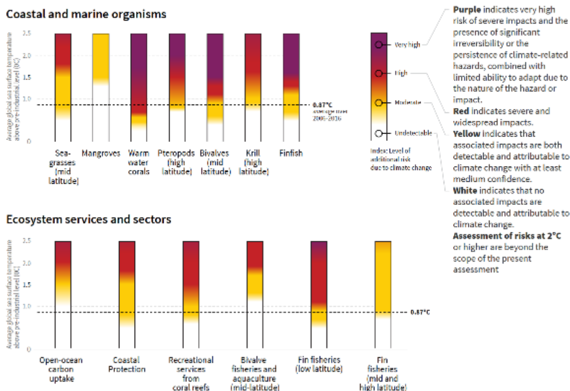
Figure 3.18: Summary of additional risks of impacts from ocean warming (and associated climate change factors such as ocean acidification) for a range of ocean organisms, ecosystem and sectors at 1.0°C, 1.5°C and 2.0°C warming of average sea surface temperature (SST) relative to the preindustrial period. The dotted line (0.87°C) is a measure of the extent of present day warming. Assessment of changing risk levels and associated confidence were derived from the expert judgement of Gattuso et al., (2015) and the Lead Authors of this Chapter plus the additional input was received from the many reviewers of the ocean systems section of SR1.5. Note: (1) The analysis done here is not intended to be comprehensive. The examples of organisms, ecosystems and sectors discussed here are intended to outline the evidence and projection of impacts and the risks for ocean systems. (2) The evaluation of risks by experts did not consider genetic adaptation, acclimatization, or human risk reduction strategies (mitigation and societal adaptation). (3) As discussed elsewhere (3.3.10, 3.4.4.5, Box 3.4; Gattuso et al 2015), ocean acidification
