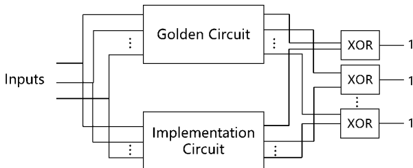
Fig. 1. Construction of miter circuits. A miter circuit is constructed by connecting the output gates of golden circuit and of implementation circuit to a group of exclusive-OR (XOR) gates.
