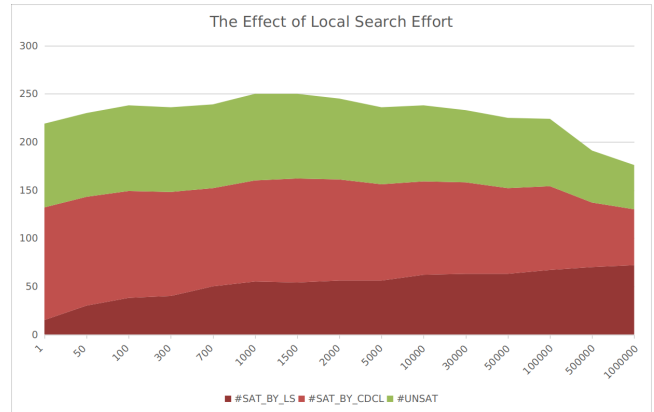
Fig. 1. The Effect of Local Search Effort on SAT Solving.
