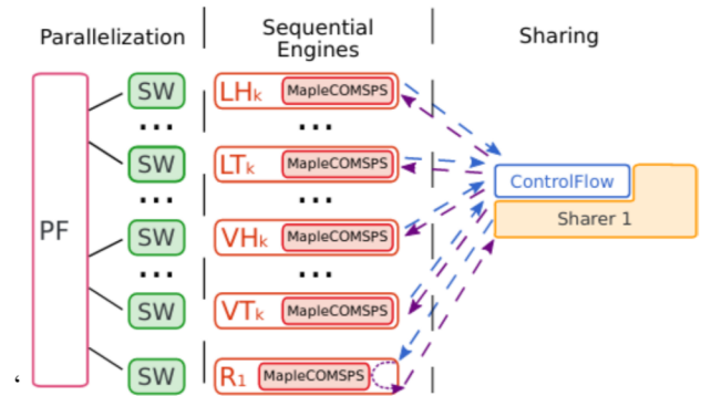
Fig. 1. Architecture of P-MCOMSPS
