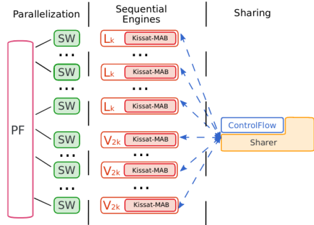
Fig. 1. Architecture of P-KISSAT-MAB
